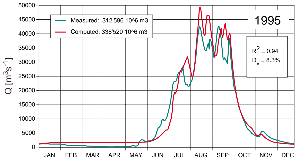
Figure 4: Measured and computed runoff in the river Ganges, 1995
