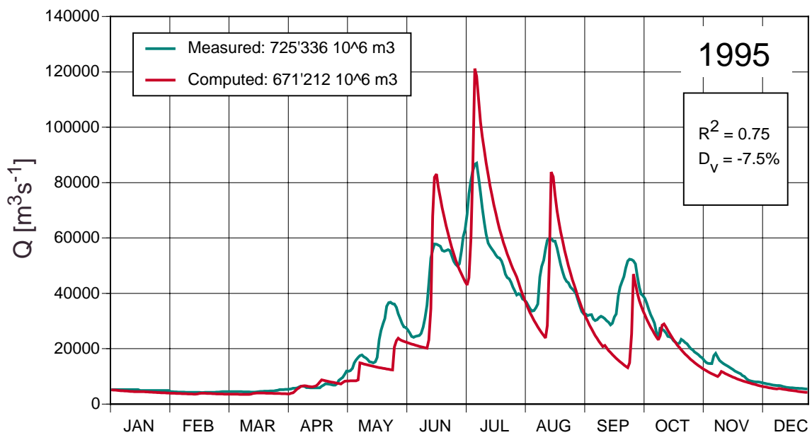
Figure 5: Measured and computed runoff in the river Brahmaputra, 1995
