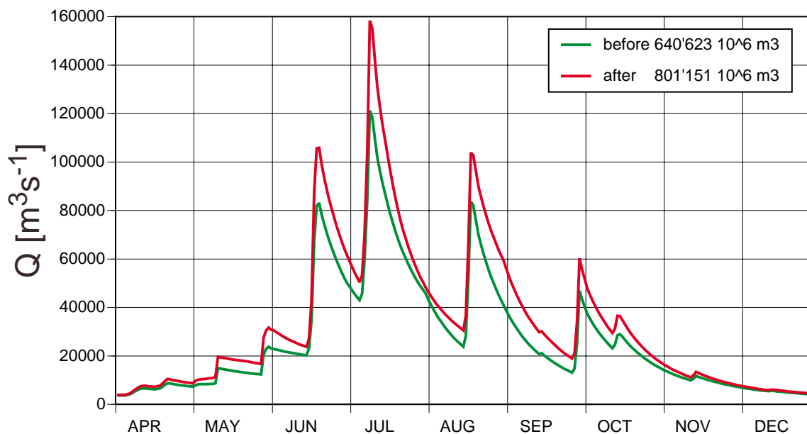
Figure 10: Computed (1995) and climate affected runoff in the basin of Brahmaputra
