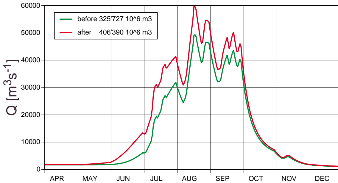
Figure 9: Computed (1995) and climate affected runoff in the basin of Ganges
