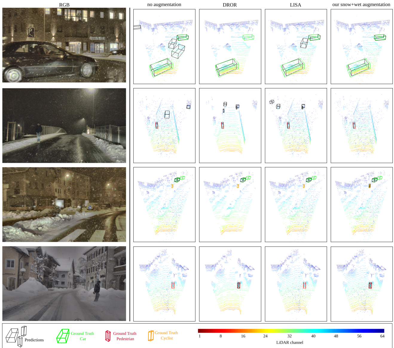
Figure 11. Qualitative comparison of PV-RCNN [13] on samples from STF [1] containing heavy snowfall. The leftmost column shows the corresponding RGB images. The rest of the columns show the LiDAR point clouds with ground-truth boxes and predictions using the clear-weather baseline (“no augmentation”), DROR [3], LISA [9], and our fully-fledged simulation (“our snow+wet augmentation”). Best viewed on a screen and zoomed in.
