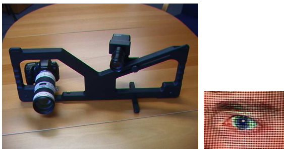
Figure 4: Left: The ShapeCam system consists of a flash projecting a grid and a camera. The camera takes an image from a direction that is slightly different from the direction of projection. Right: A regular square pattern is projected on the scene, as seen in this detailed view. 3D co-ordinates are calculated for all the line intersections, resulting in the simultaneous measurement for thousands of points.
